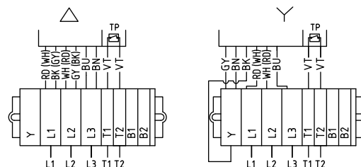
3-Ph motor dual voltage with TP
