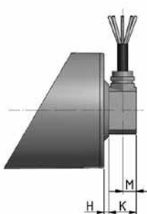
Cable connection 90°.
