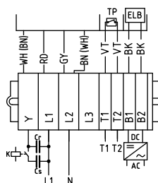
1-Ph motor with TP & ELB
