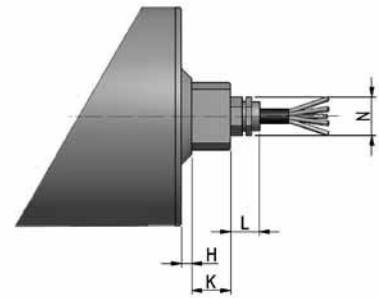
Straight connector.
